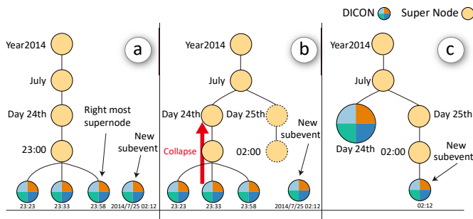
Fig. 4. (a) A new subevent arrives. (b) The node of Day 24th is collapsed, and the two super nodes of Day 25th and 02:00 are added. (c) The new subevent is added as the rightmost leaf of the tree.
