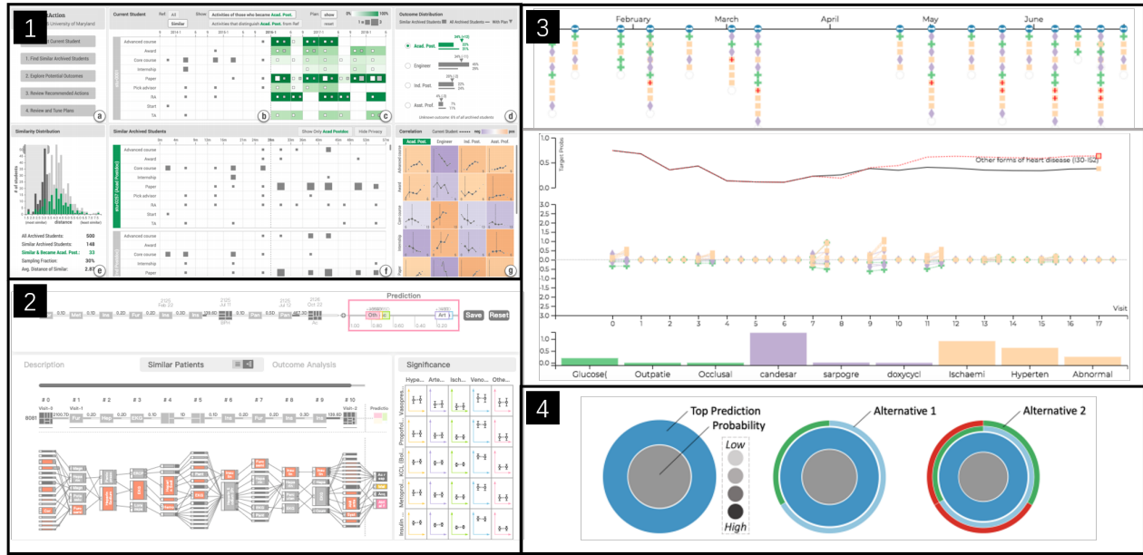
Fig. 4. Selected examples of visual prediction & recommendation techniques. (1) EventAction [22] uses a calendar view to show the temporal information of event sequences. (2) CarePre [48] reveals the medical record of a patient in a timeline-based visualization, and similar patients' medical event sequences are aggregated into a Sankey-based visualization. (3) In RetainVIS [60], predicted risk trajectories are revealed in parallel line charts (middle), and the risk contributors for the patients are displayed in a bar chart (bottom). (4) [37] visualizes the top prediction, alternatives, and their uncertainties in a circular glyph design.
